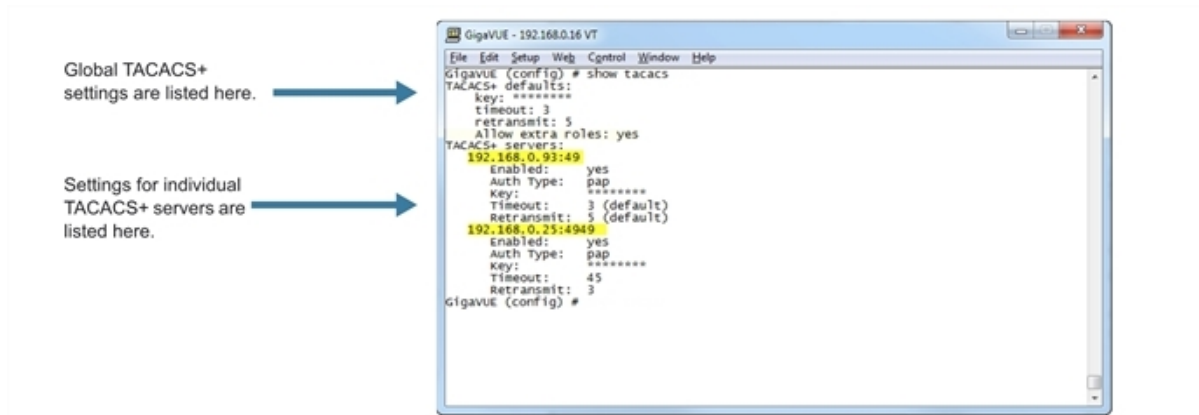
Figure 29 Results of show tacacs Command
